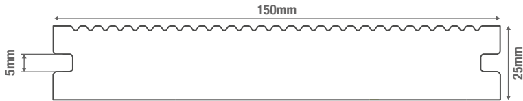
Solid Composite Decking Board
