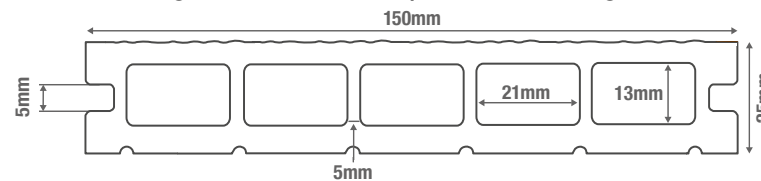
Woodgrain Effect Composite Decking Board
