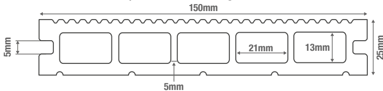
Hollow Composite Decking Board
