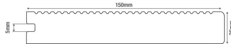
Bullnose Composite Decking Board
